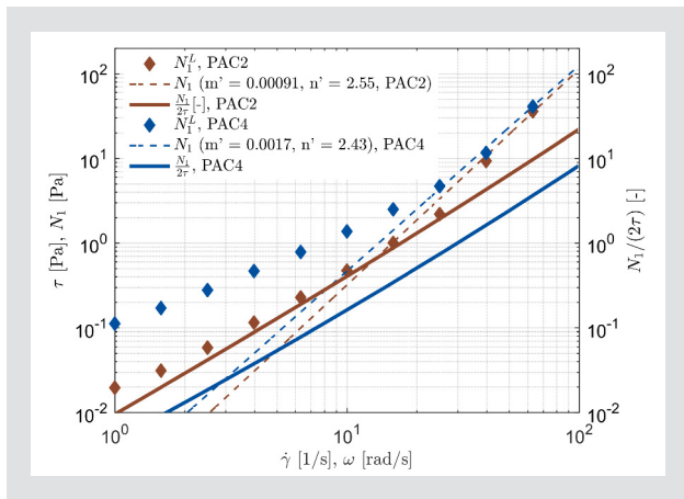
Figure 10: PAC2 and PAC4 recoverable shear N_1/(2\tau) , where the FNSD N_1 is based on PL fits to the FNSD N_1^t = \psi_1 \dot{\gamma}^2 and the FNSC \psi_1 is obtained from FS data via Laun's rule [44].
