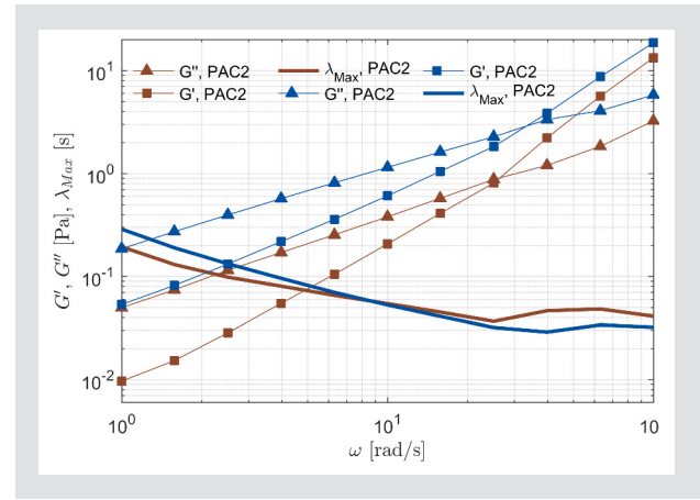
Figure 5: Frequency sweeps ( \gamma = 0.2 \% ) for PAC2 and PAC4.
