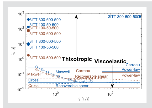
Figure 11: PAC2 and PAC4 time scales overview.
